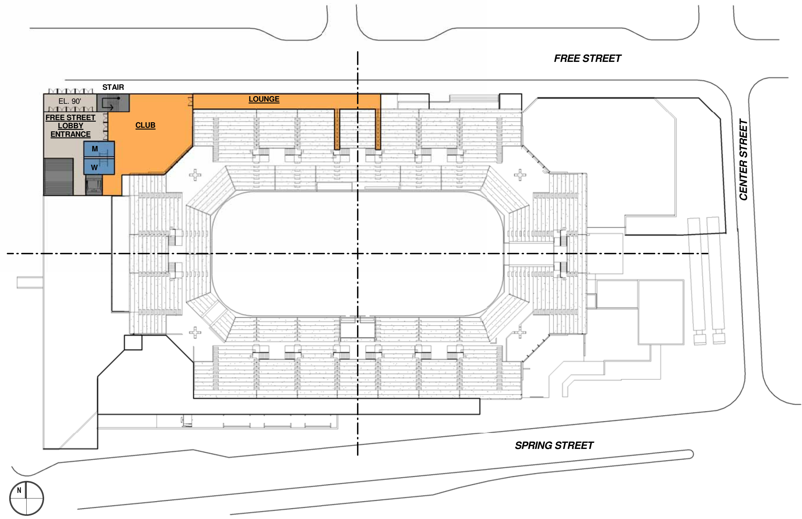
① 03.5 - FREE STREET NW ENTRANCE - FLOOR PLAN 1" = 40'-0" 0 20 40 80
