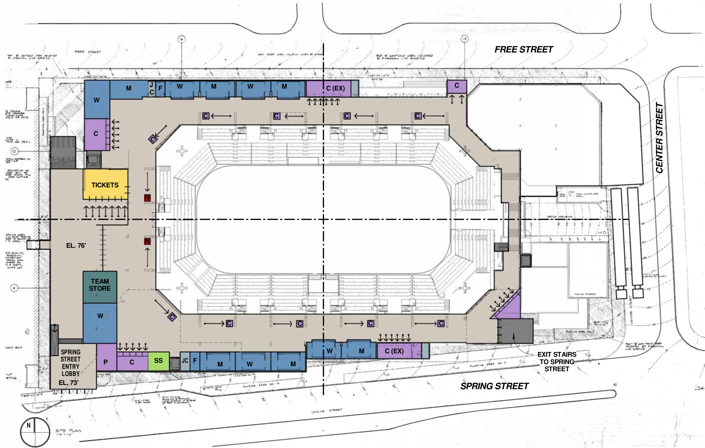
① 03 - MAIN CONCOURSE - FLOOR PLAN 1" = 40'-0" 0 20 40 80
