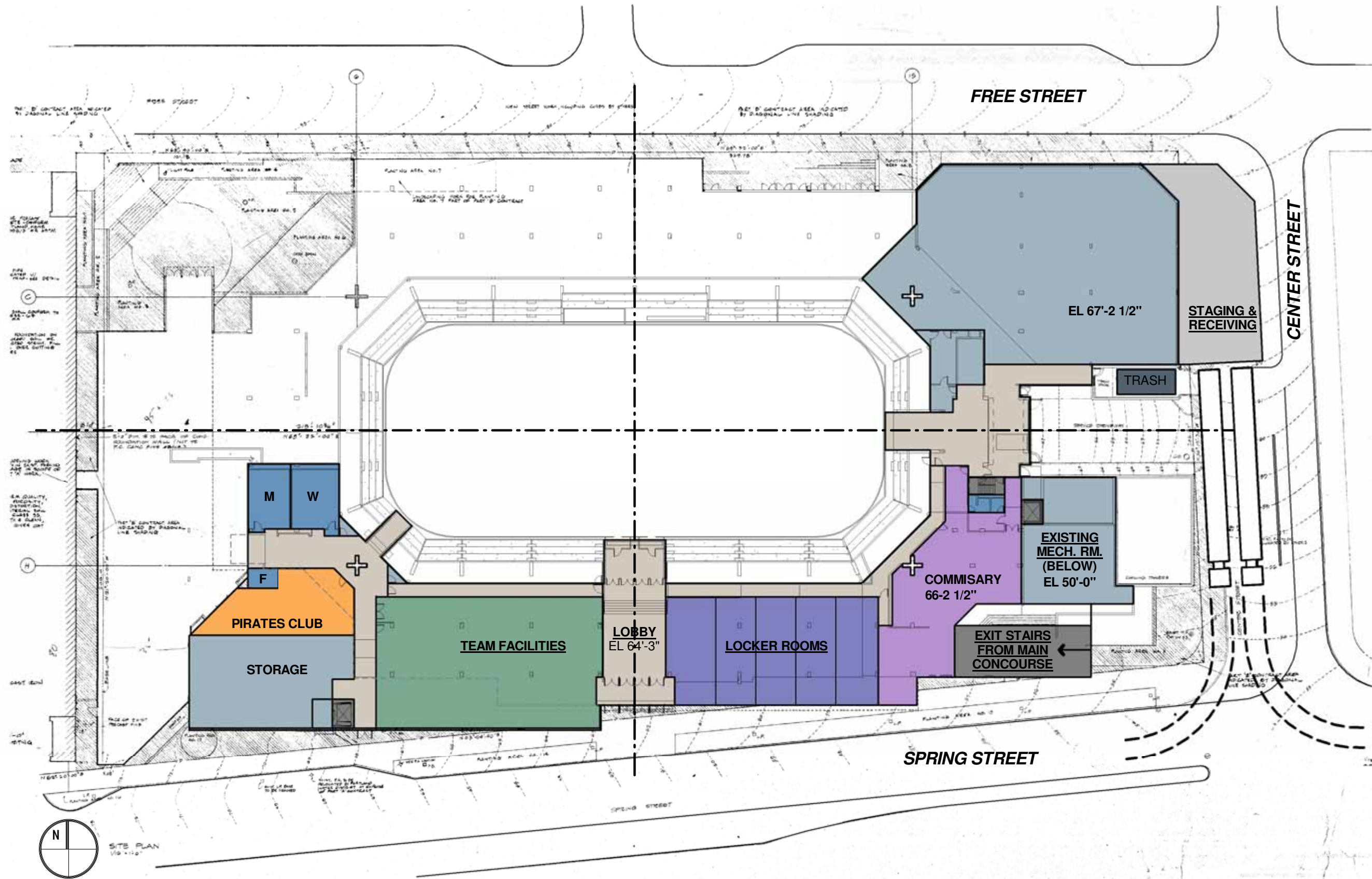
① 01 - EVENT LEVEL - FLOOR PLAN 1" = 40'-0" 0 20 40 80
